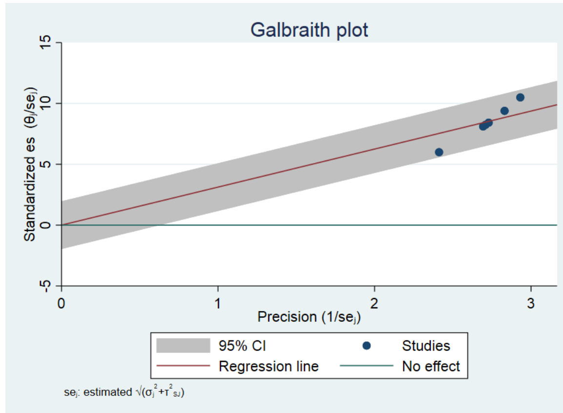
Supplementary Fig. 3. Galbraith plot of the mean vitamin D level. CI. confidence interval.
